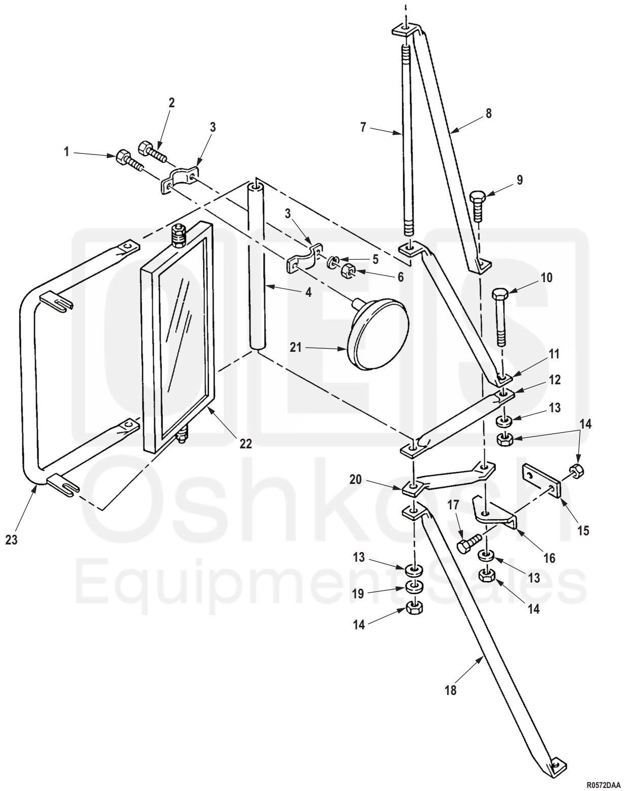
Figure 555. Rearview Mirrors.
